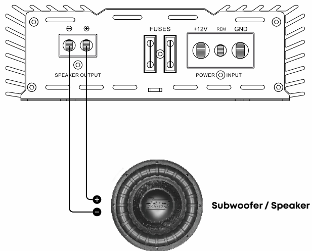
1 Ch Monoblock
