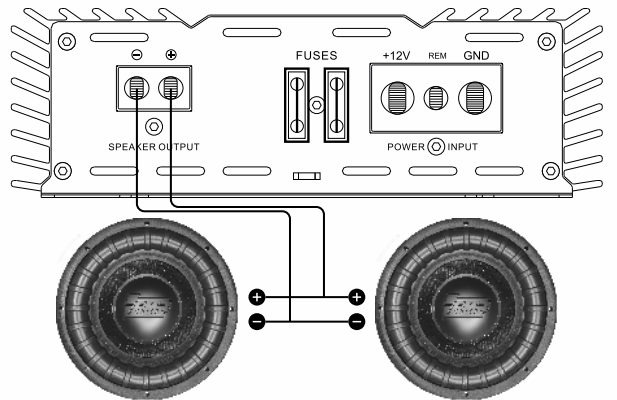
1 Ch Monoblock
