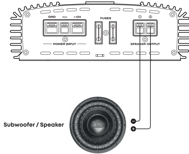
1 Ch Monoblock
