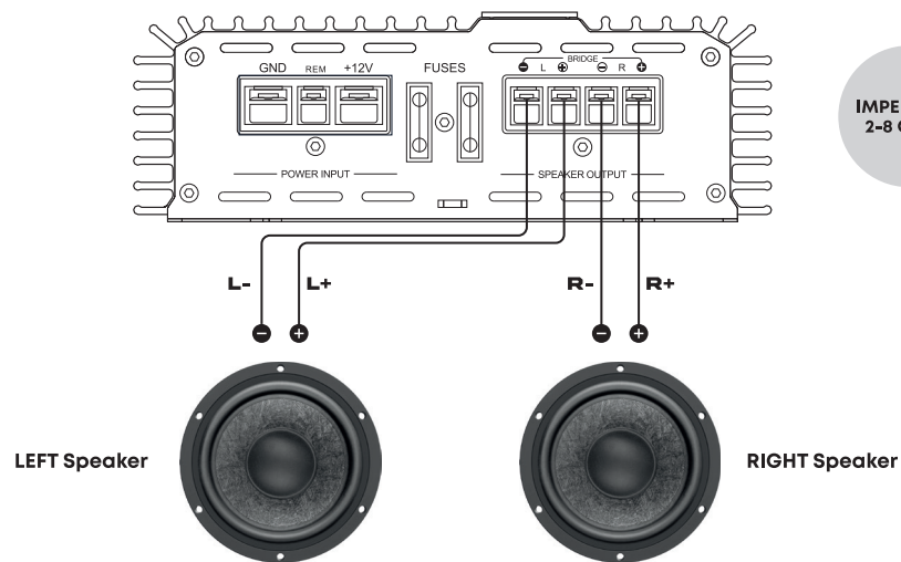
2 Channel amplifier
