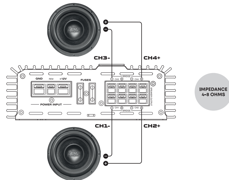
Bridge Mode
