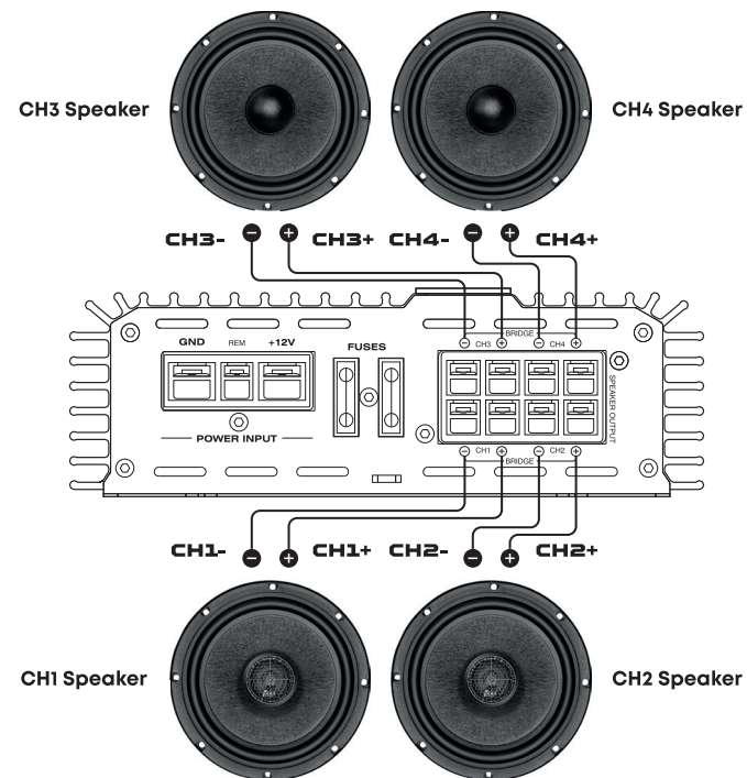
4 Channel amplifier
